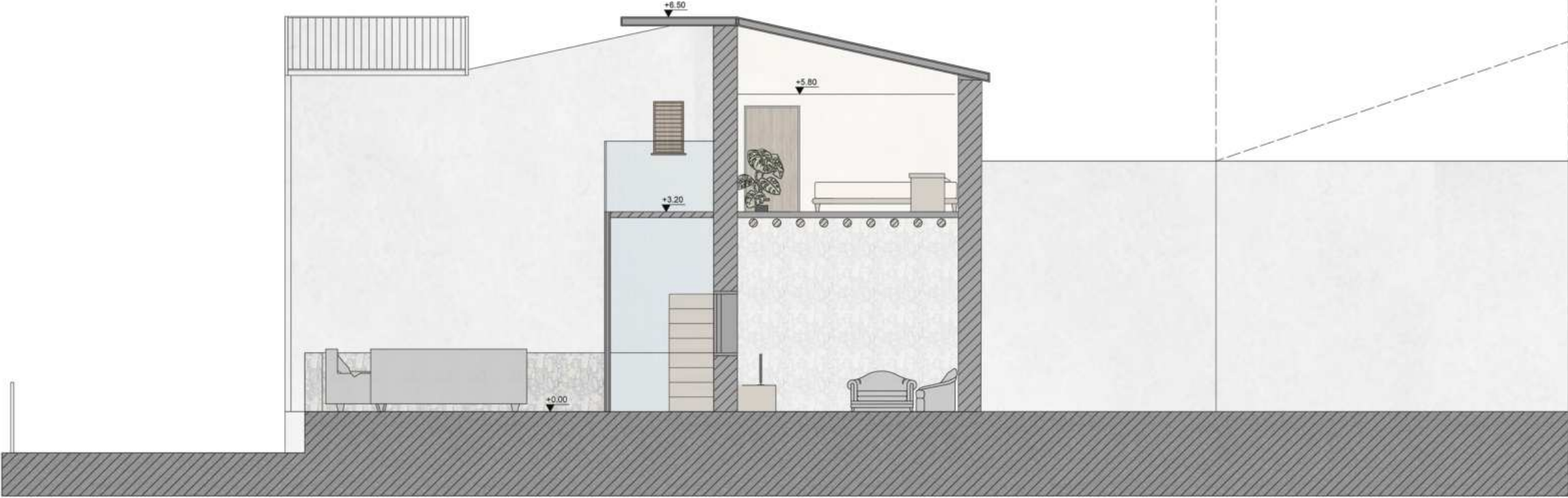
SECTION B-B'
